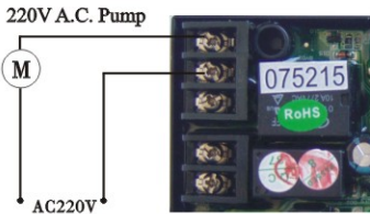
Figure3-7 Wiring diagram of inlet pressure pump (<5A)
