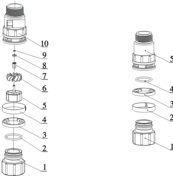
5447007 Flow Meter
