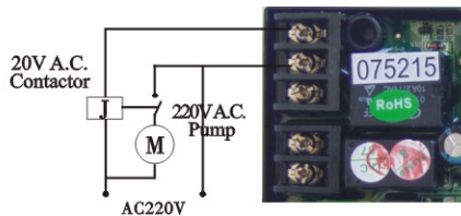
Figure3-8 Wiring diagram of inlet pressure pump (<5A)
