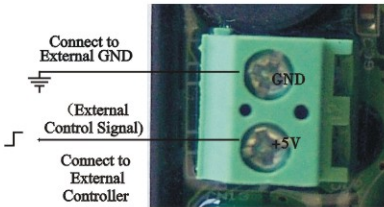
Figure 3-11 Wiring of Remote Handling Connector
