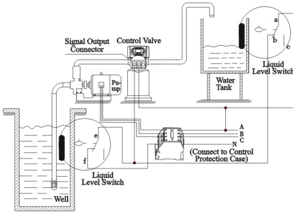
Figure3-6 Wiring of Liquid Level Switch in Water Tank Controls Inlet
