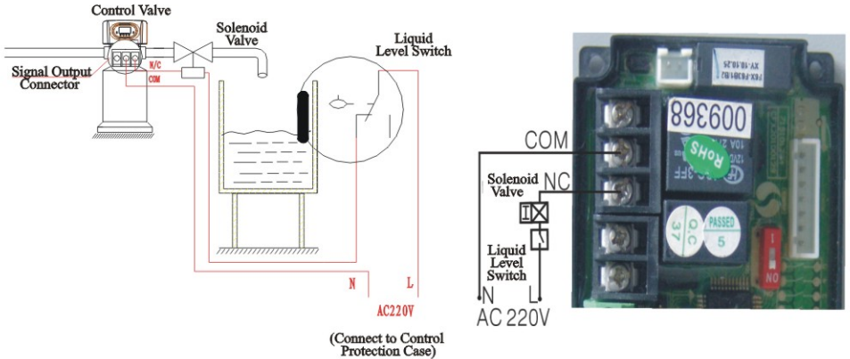
Figure3-2 Wiring of Outlet Solenoid Valve
